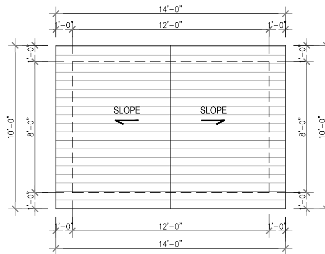
2 ROOF FLOOR PLAN Scale 1"=1/4"
