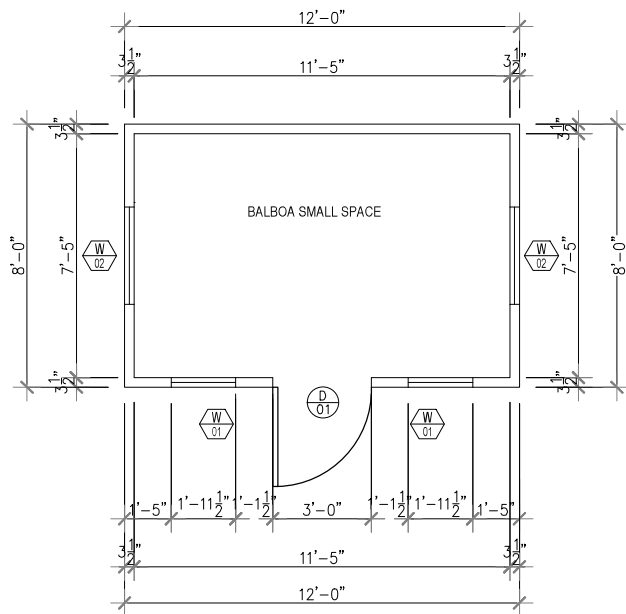
1 GROUND FLOOR PLAN Scale 1"=1/4"
