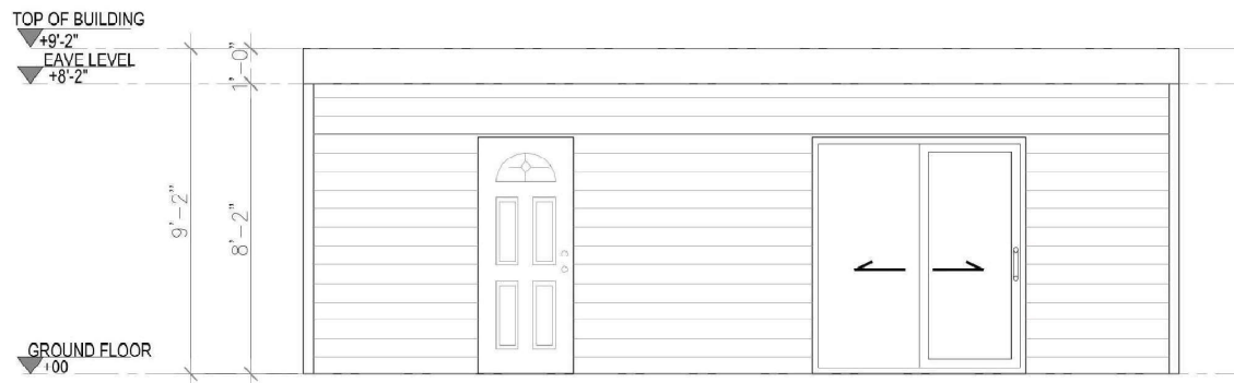
1 FRONT ELEVATION Scale 1'=1/4"
