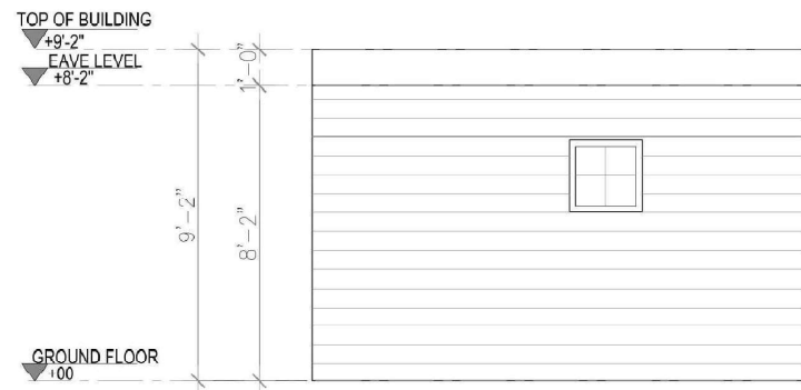
3 RIGHT SIDE ELEVATION Scale 1'=1/4"
