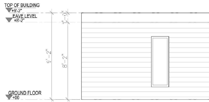
4 LEFT SIDE ELEVATION Scale 1'=1/4"
