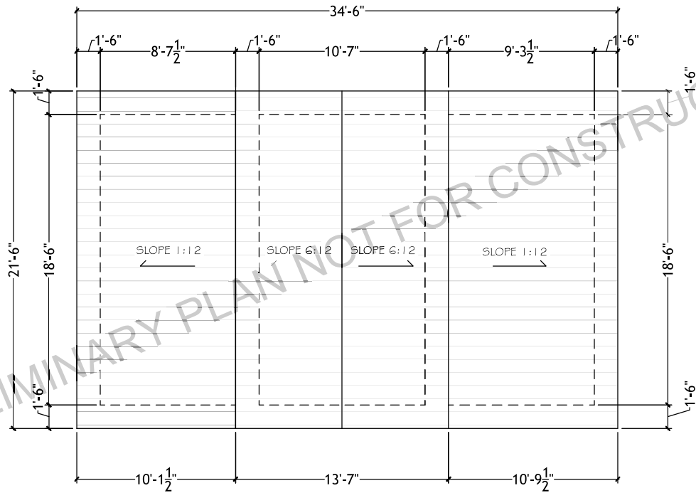
ROOF PLAN SCALE: 1"=1/4"
