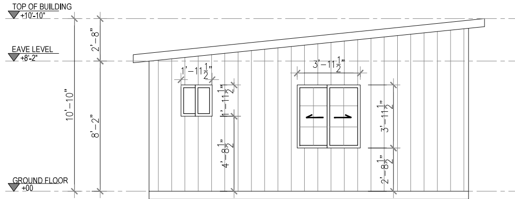
2 LEFT SIDE ELEVATION Scale 1"=1/4"
