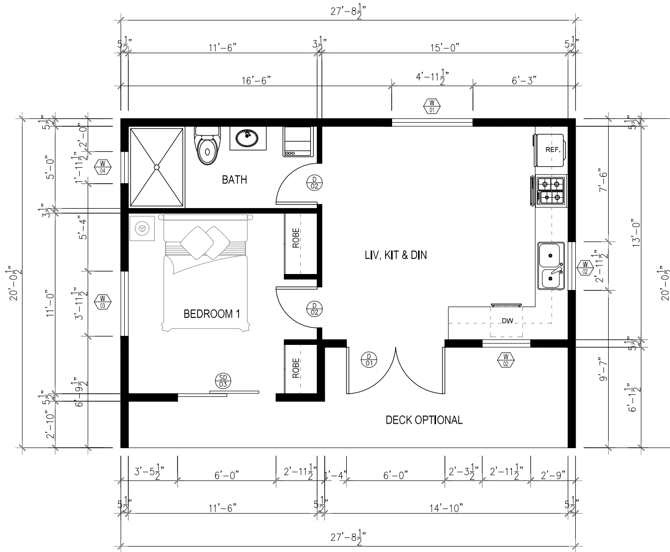
1 GROUND FLOOR PLAN Scale 1"=1/4"
