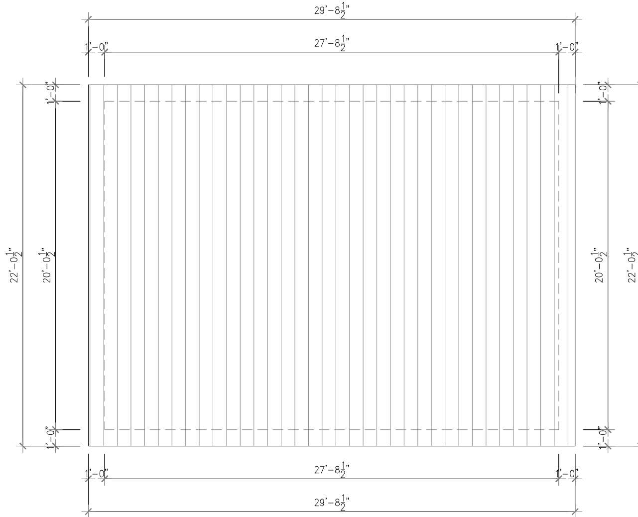
1 ROOF FLOOR PLAN Scale 1"=1/4"
