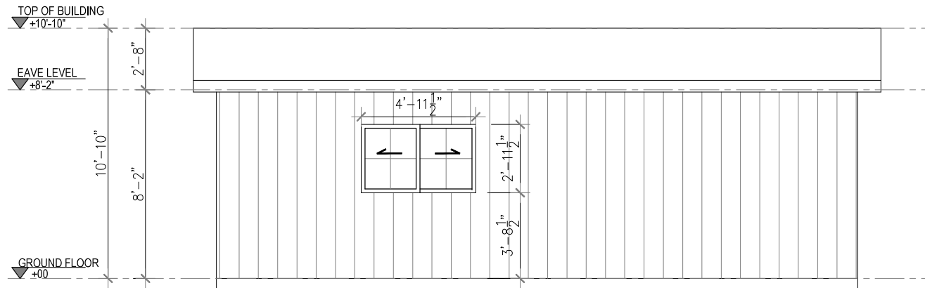
2 REAR ELEVATION Scale 1"=1/4"
