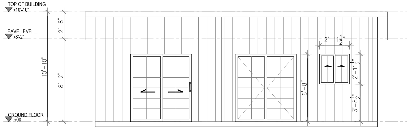
1 FRONT ELEVATION Scale 1"=1/4"
