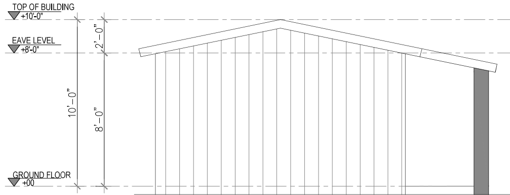
3 LEFT SIDE ELEVATION Scale 1"=1/4"
