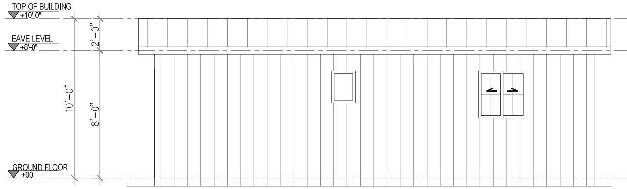
2 REAR ELEVATION Scale 1"=1/4"
