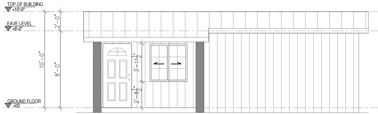
1 FRONT ELEVATION Scale 1"=1/4"
