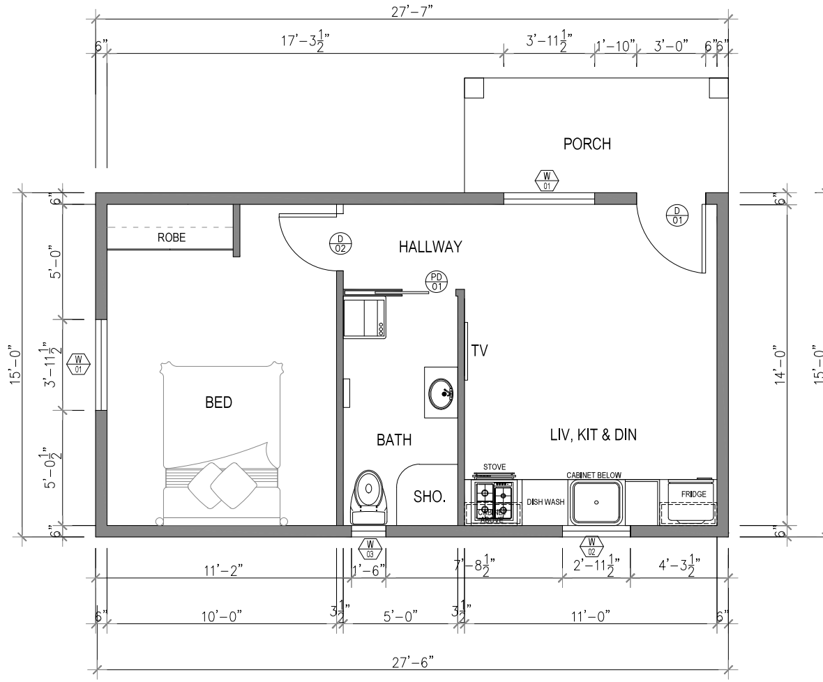
1 GROUND FLOOR PLAN Scale 1"=1/4"
