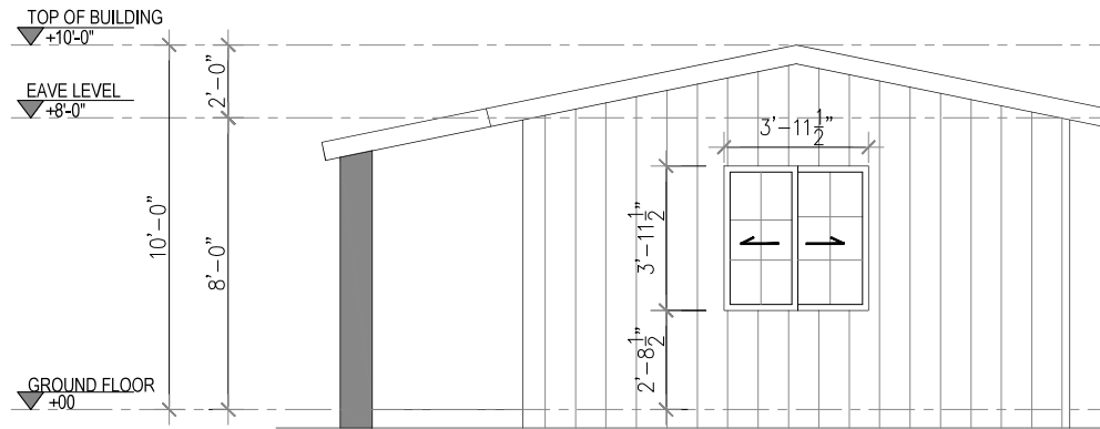
4 RIGHT SIDE ELEVATION Scale 1"=1/4"
