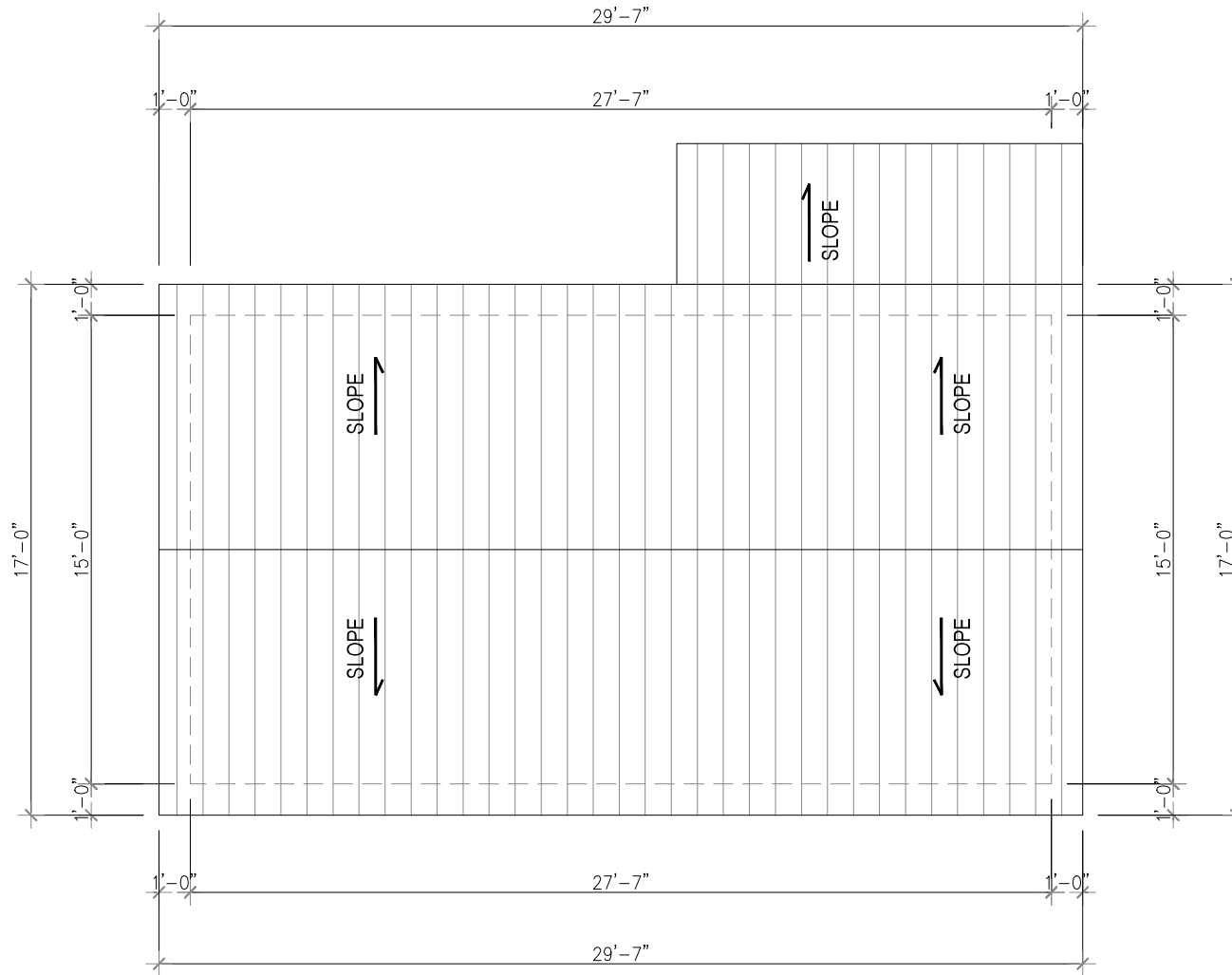
1 ROOF FLOOR PLAN Scale 1"=1/4"
