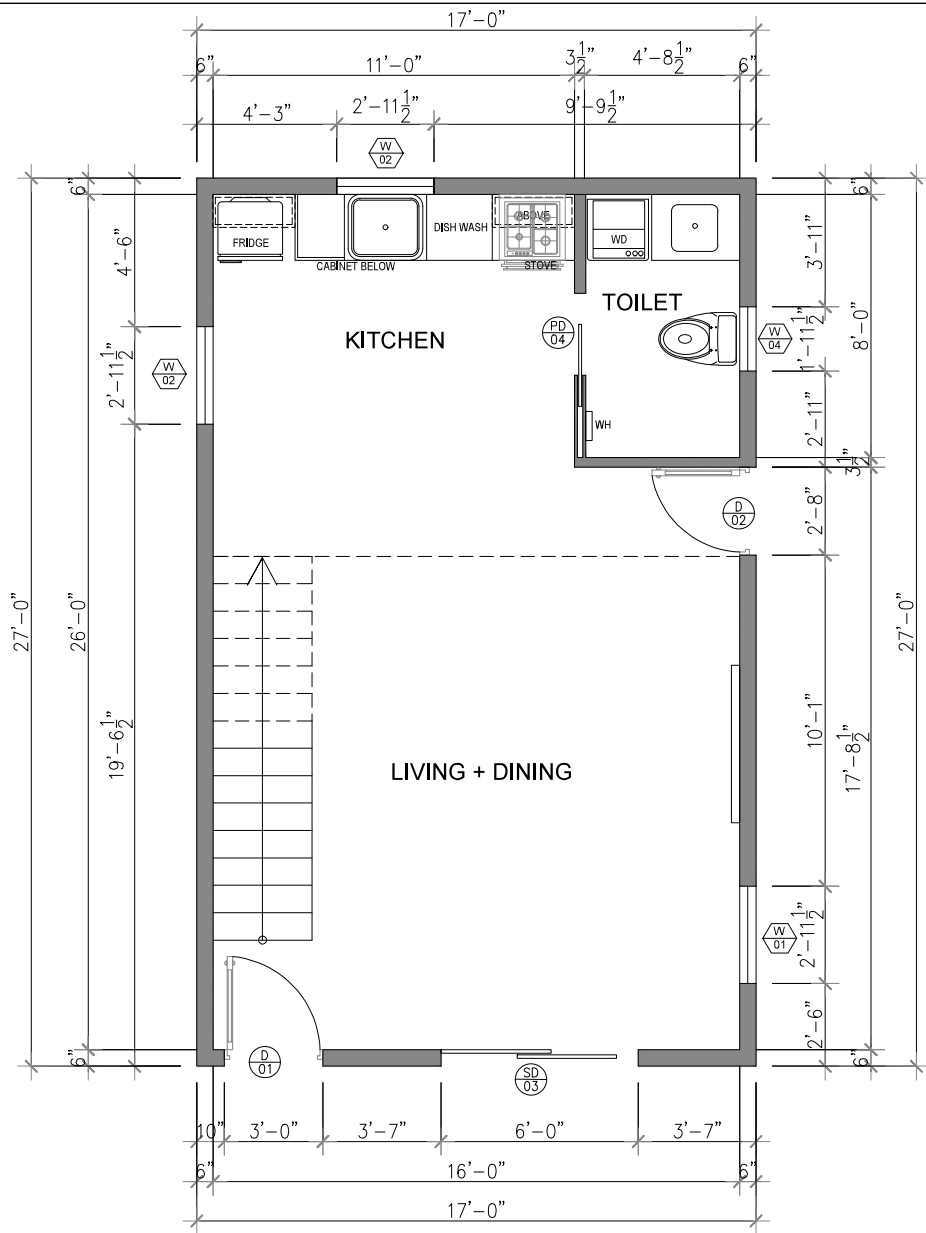
1 GROUND FLOOR PLAN SCALE= 1"=1/4"
