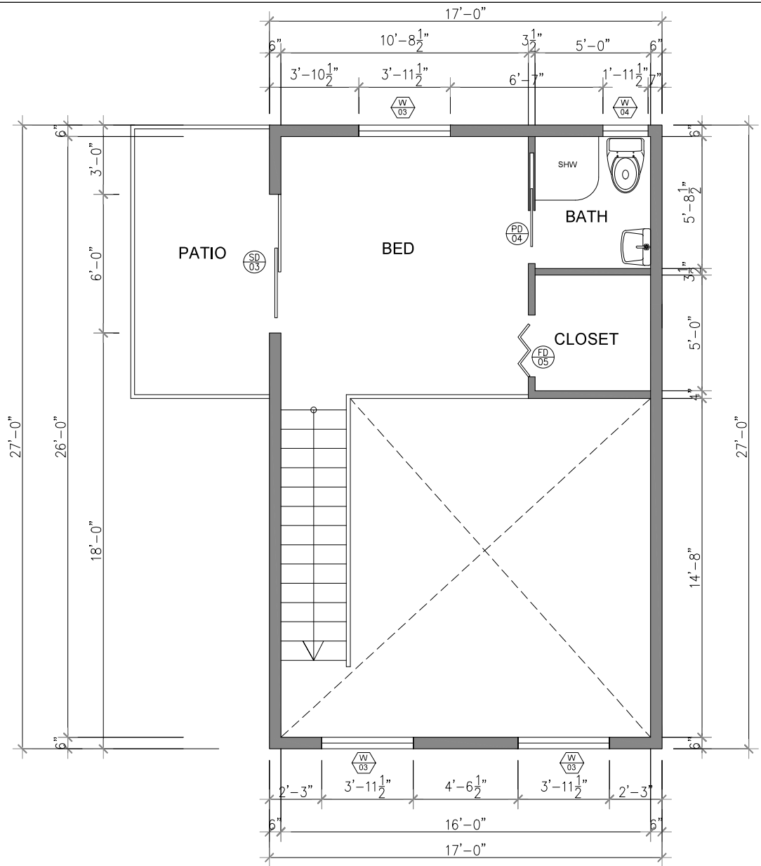
2 FIRST FLOOR PLAN SCALE= 1"=1/4"
