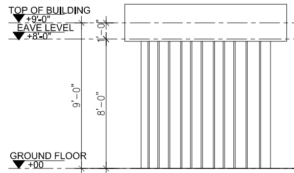
4 LEFT SIDE ELEVATION Scale 1'=1/4"
