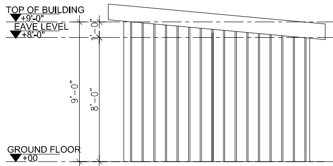
1 REAR ELEVATION Scale 1'=1/4"
