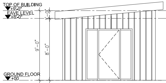
1 FRONT ELEVATION Scale 1'=1/4"
