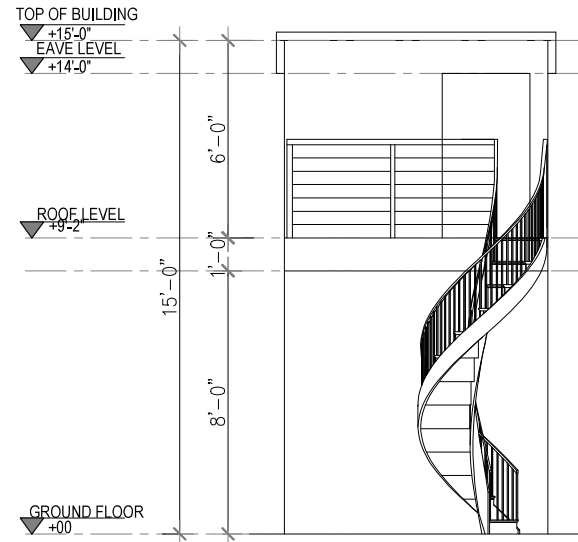
4 LEFT ELEVATION Scale 1"=1/4"
