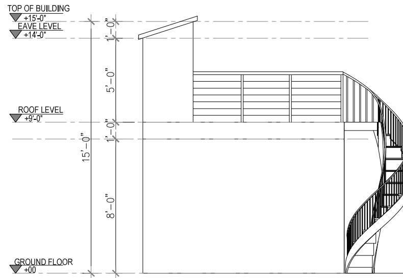
2 BACK ELEVATION Scale 1"=1/4"
