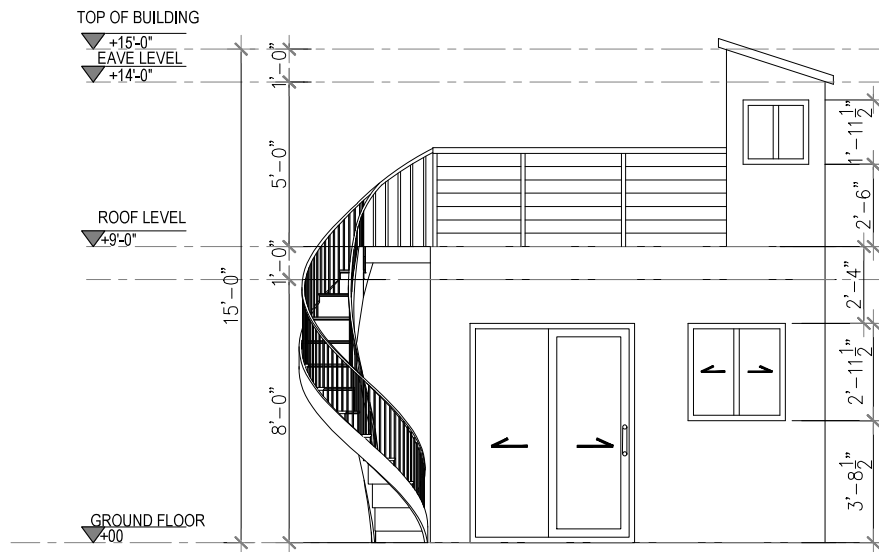
1 FRONT ELEVATION Scale 1"=1/4"
