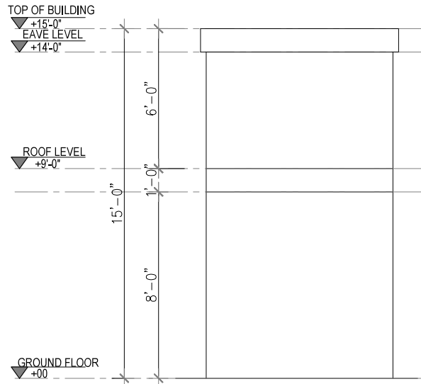
3 RIGHT ELEVATION Scale 1"=1/4"
