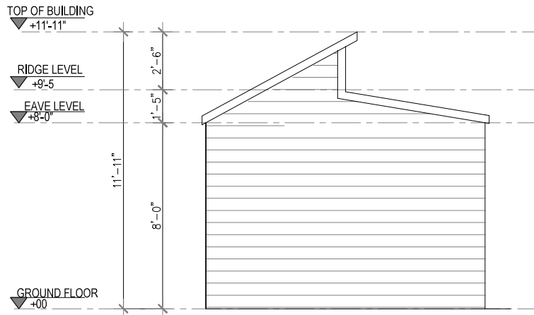
2 REAR ELEVATION Scale 1"=1/4"
