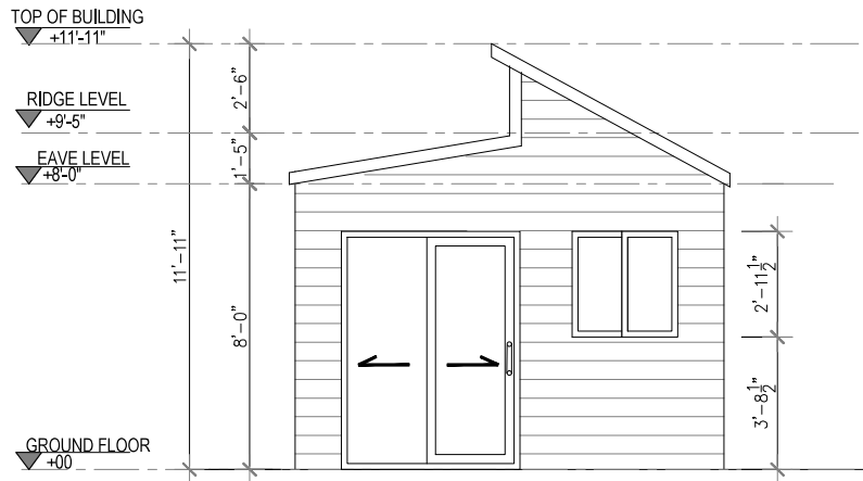
1 FRONT ELEVATION Scale 1"=1/4"
