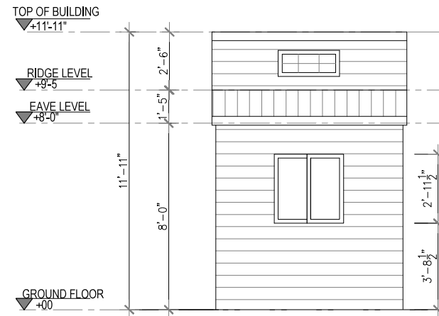
4 LEFT SIDE ELEVATION Scale 1"=1/4"
