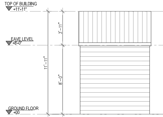
3 RIGHT SIDE ELEVATION Scale 1"=1/4"
