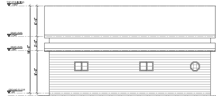
3 RIGHT SIDE ELEVATION Scale 1"=1/8"
