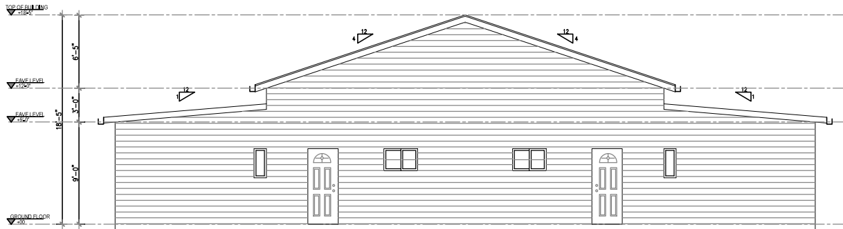
2 REAR ELEVATION Scale 1"=1/8"
