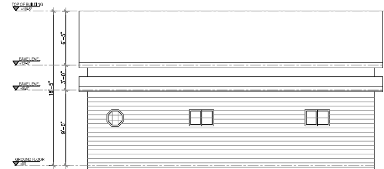
4 LEFT SIDE ELEVATION Scale 1"=1/8"
