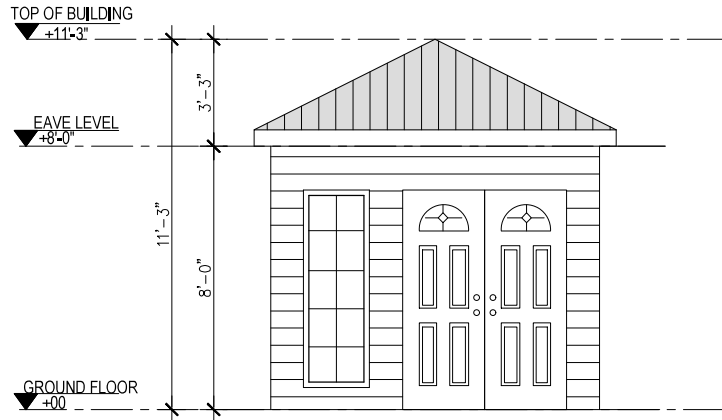
1 FRONT ELEVATION Scale 1"=1/4"
