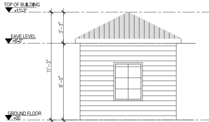
4 LEFT SIDE ELEVATION Scale 1"=1/4"
