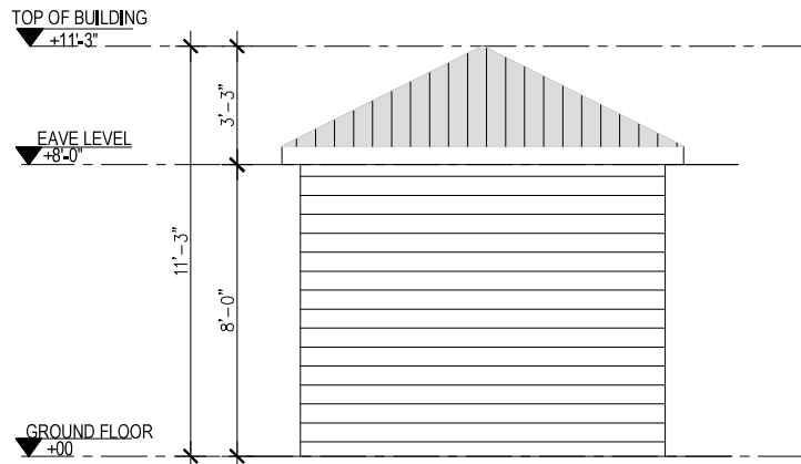
2 REAR ELEVATION Scale 1"=1/4"
