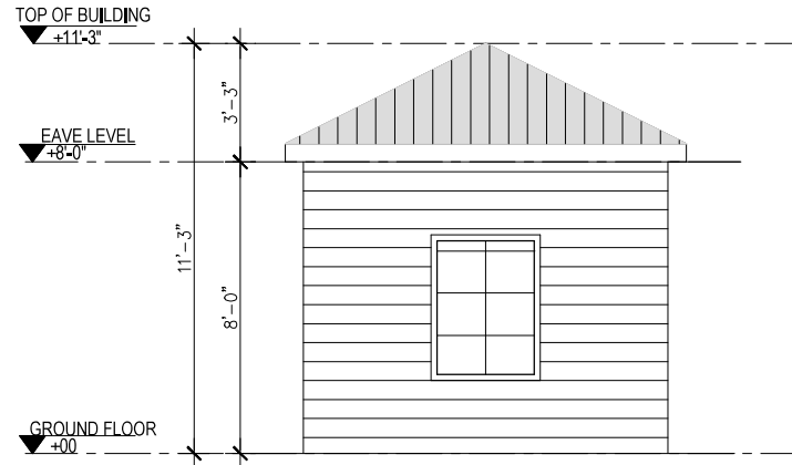
3 RIGHT SIDE ELEVATION Scale 1"=1/4"
